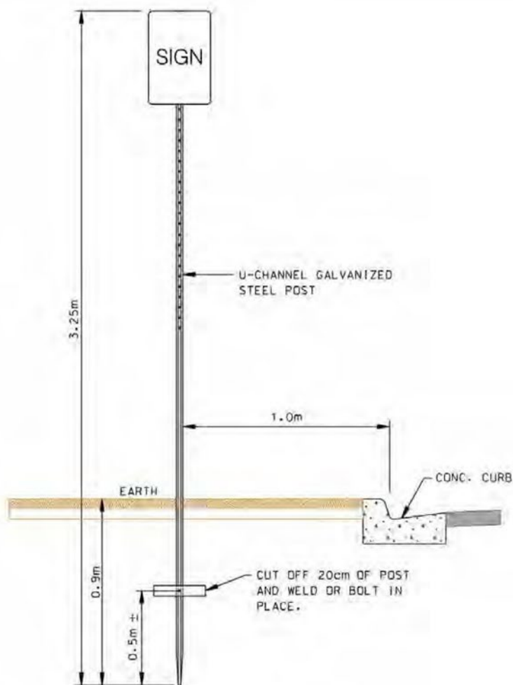
U-CHANNEL POST DETAIL
