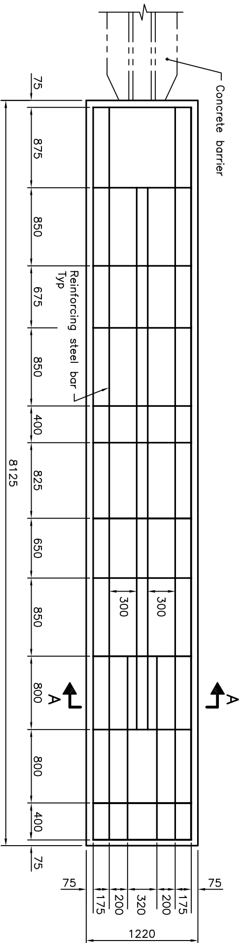
CONCRETE PAD FOR TL-3 SYSTEM CONFIGURATION
