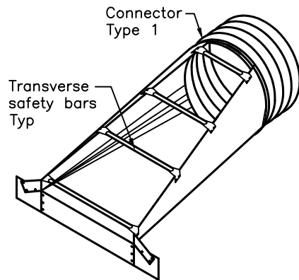
PARALLEL DRAINAGE STRUCTURE
