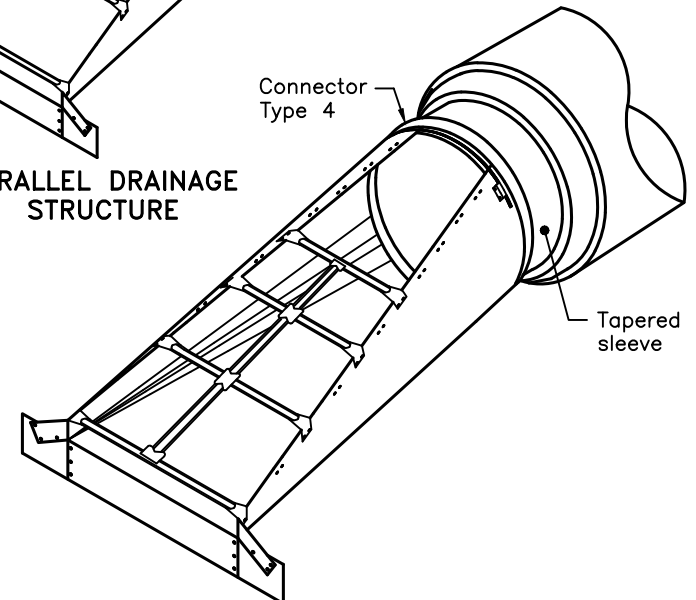
CROSS DRAINAGE STRUCTURE CIRCULAR SMOOTH WALLED AND ELLIPTICAL PIPES Concrete Pipe Shown
