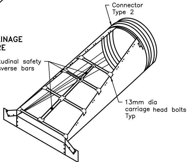
CROSS DRAINAGE STRUCTURE CIRCULAR AND ARCHED CORRUGATED PIPES
