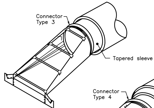
PARALLEL DRAINAGE STRUCTURE
