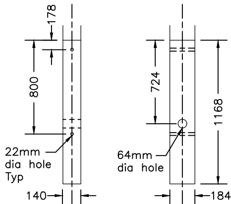
FRONT VIEW SIDE VIEW BREAKAWAY WOODEN POST
