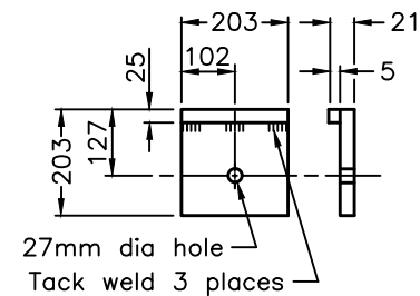
STEEL BEARING PLATE DETAIL
