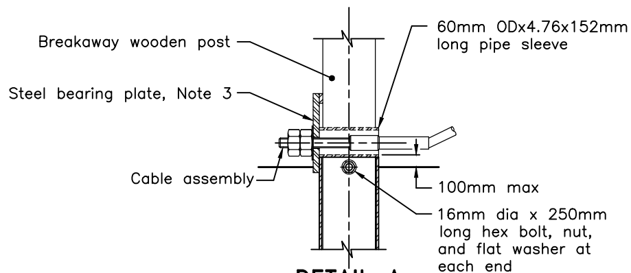
DETAIL A (STRUTS NOT SHOWN FOR CLARITY)
