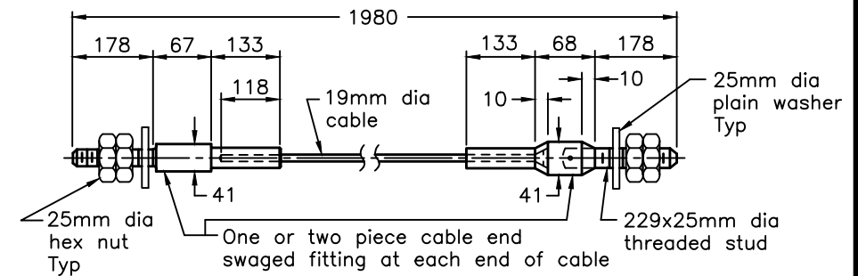
ONE PIECE CABLE END TWO PIECE CABLE END
