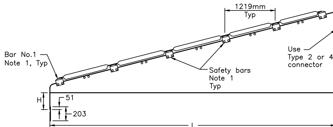
SIDE VIEW FOR CROSS DRAINAGE STRUCTURE
