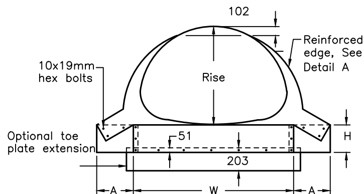
FRONT VIEW ARCHED PIPE
