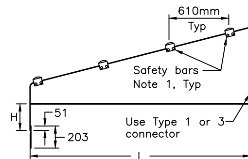
SIDE VIEW OF PARALLEL DRAINAGE STRUCTURE
