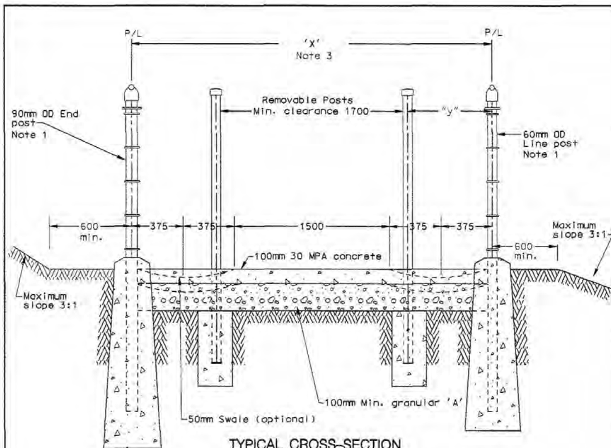
TYPICAL CROSS-SECTION
