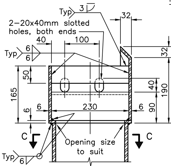
CATCH BASIN DETAILS
