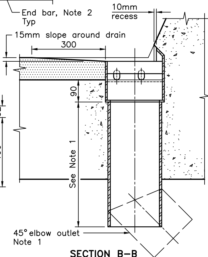
SECTION B-B
