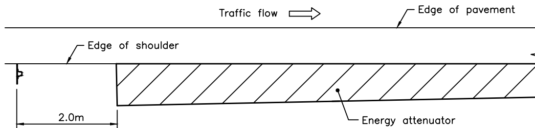
STEEL BEAM ENERGY ATTENUATING TERMINAL - FLARED
