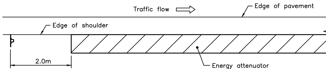
STEEL BEAM ENERGY ATTENUATING TERMINAL - TANGENT
