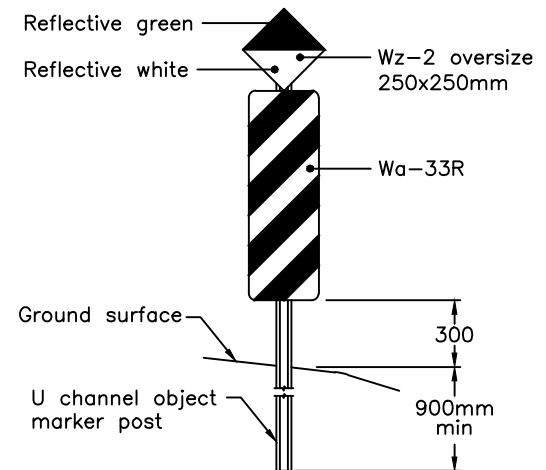
APPROACH END - RIGHT SHOULDER
