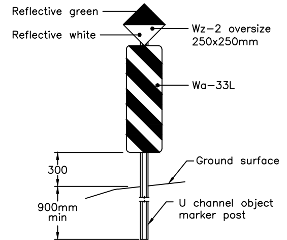
APPROACH END - LEFT SHOULDER
