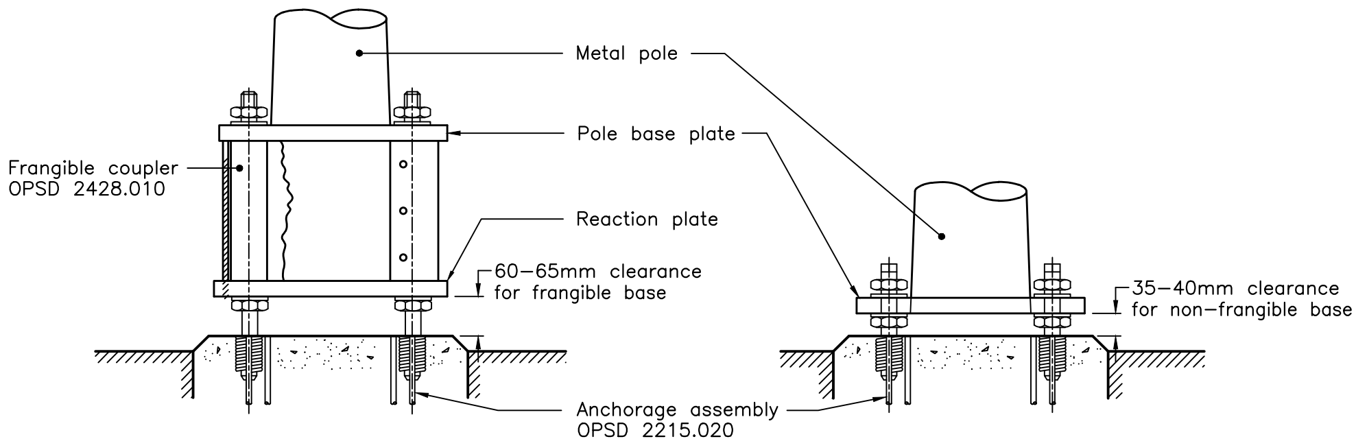
FRANGIBLE BASE - FRANGIBLE COUPLER
