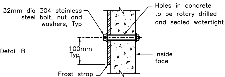
DETAIL C
