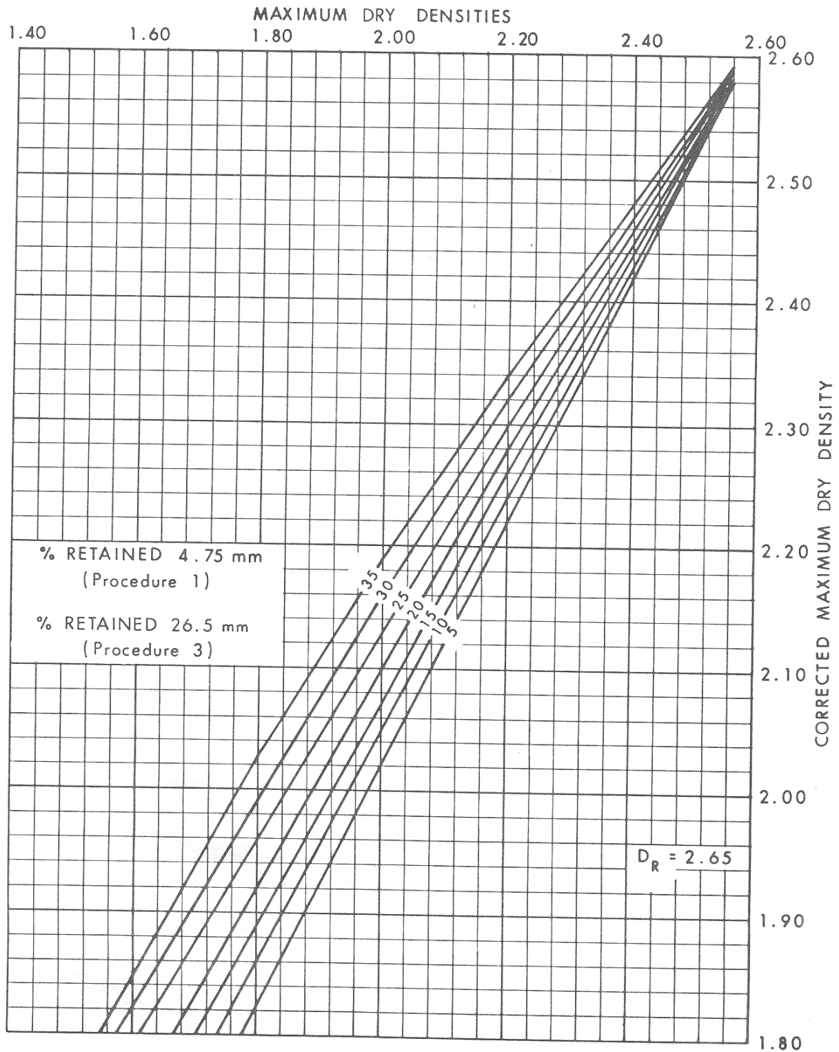
Figure 2 Plus 4.75 mm Correction Table for Dry Densities
