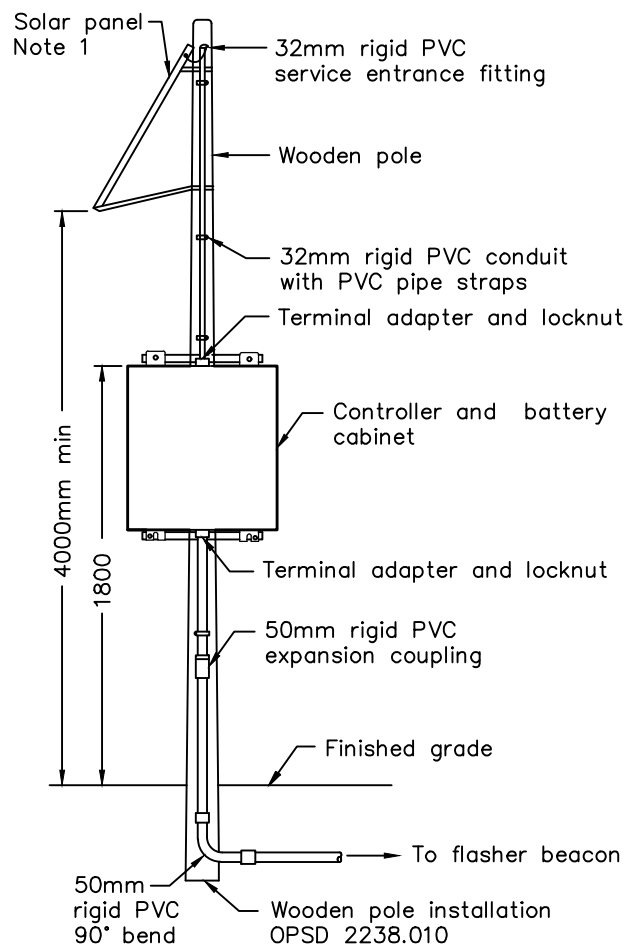
SOLAR POWER ASSEMBLY
